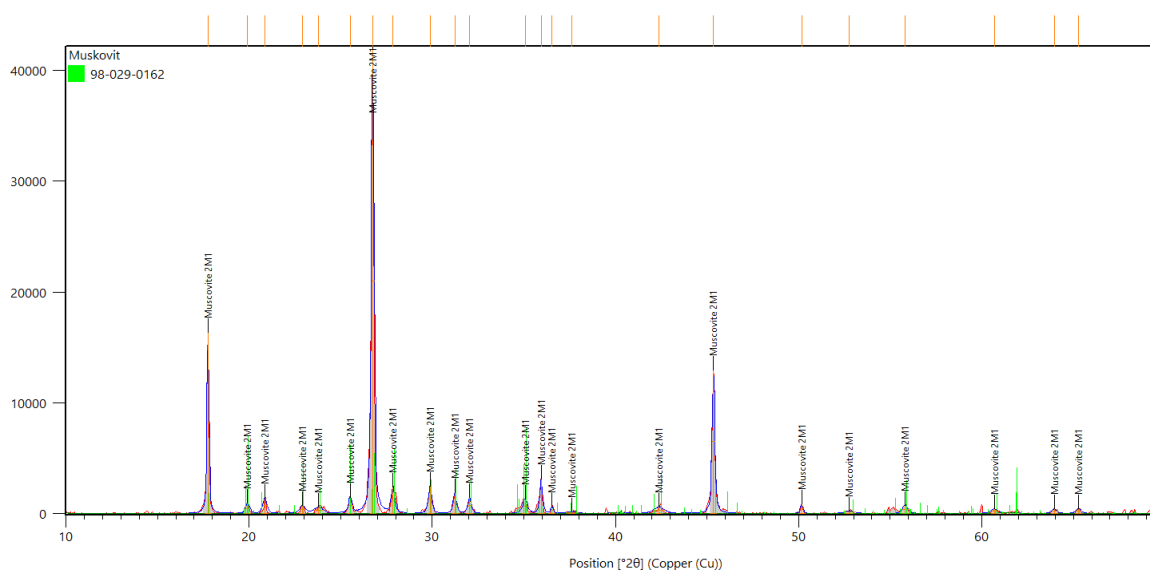
Fig. 2 X-ray diffractogram of powdered crystals confirming the identity as muscovite.
